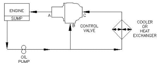
MIXING SYSTEM
