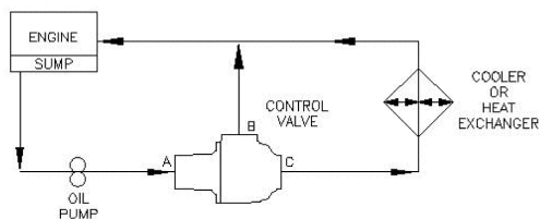
DIVERTING SYSTEM
